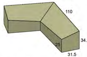
FC053 CABO SECTIONAL RIGHT COVER LL, SCC45, RL LL, SCC90, M, RL FITS: 270, 275, 4302 W: 110" D: 31.5" H: 25/34.5"
